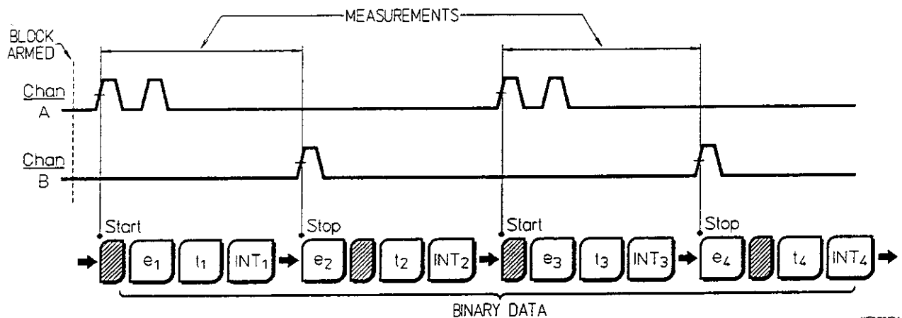
Figure 10A-A. Time Interval Measurement on Channel A → B With Automatic Arming Mode Showing Corresponding Binary Output.
