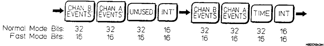
Figure 15-B. Format 15 Binary Output
