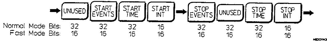
Figure 10C-B. Format 10C Binary Output
