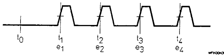
Figure 2B-E. Time Deviation and Phase Deviation Example Signal showing Time and Event Stamp Measurement Points.
