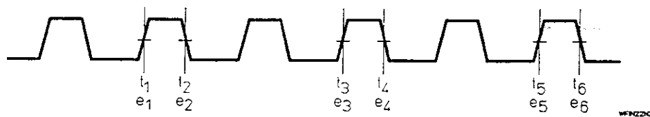
Figure 10B-D. Duty Cycle Example Signal Showing Time and Event Stamp Measurement Points
