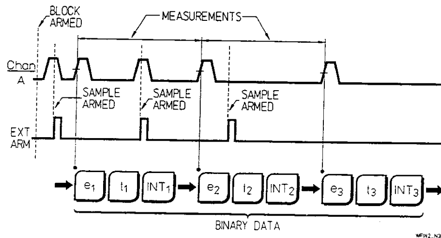
Figure 2A-A. Frequency Measurement on Channel A with Edge Sampling Arming Mode Showing Corresponding Binary Data Output.
