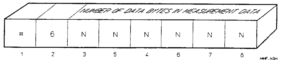
Figure 3-4. Header Format (ASCII code)
