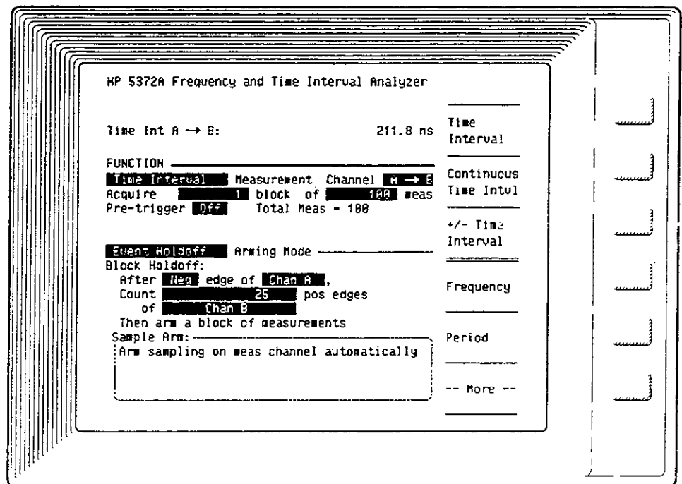
Figure D-2. Event Holdoff Arming Mode
