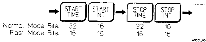
Figure 4B-B. Format 4B Binary Output
