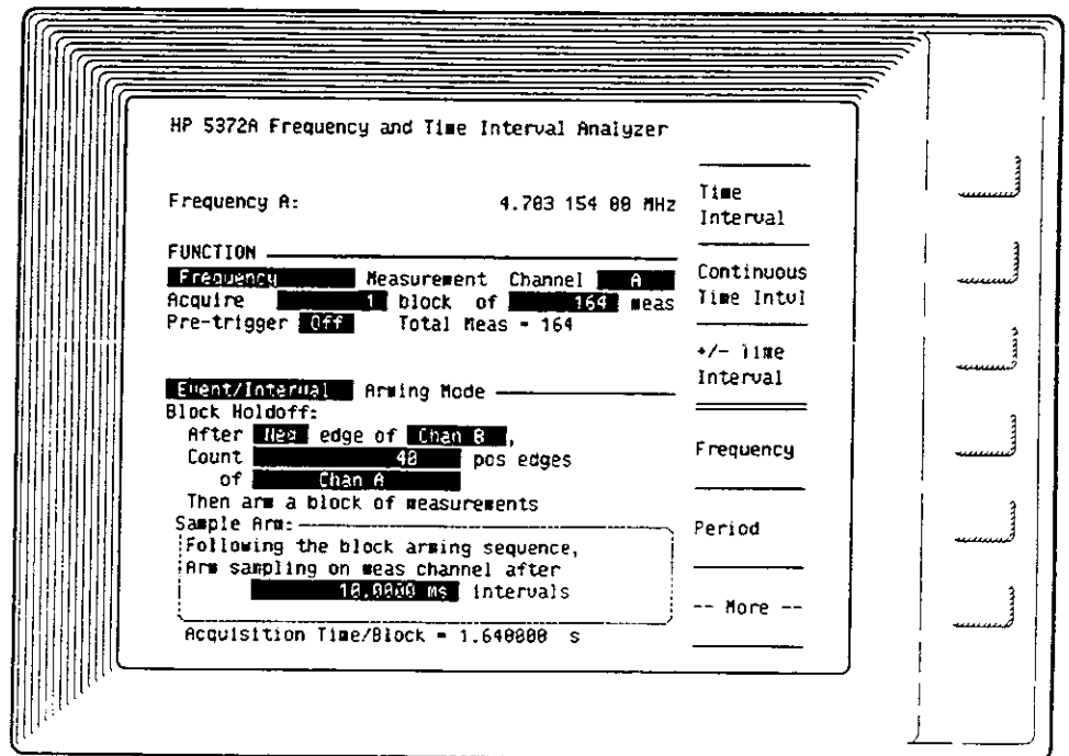
Figure D-4. Event/Interval Arming Mode
