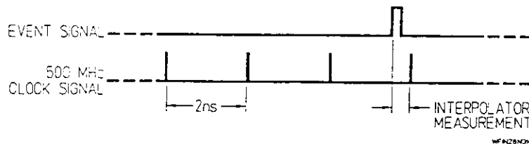
Figure 3-2. Interpolation Between 2 ns Clock Pulses
