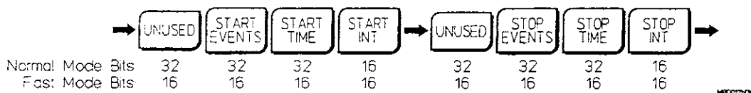
Figure 10D-C. Format 10D Binary Output: Start Before Stop
