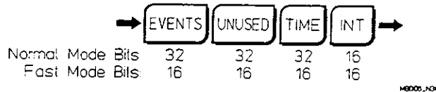
Figure 3-C. Format 3, Subsequent Samples
