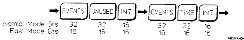
Figure 14-B. Format 14 Binary Output
