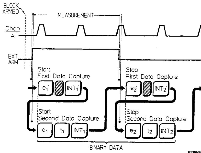
Figure 14-A. Totalize Measurement on Channel A with Externally Gated Arming Mode Showing Corresponding Binary Output
