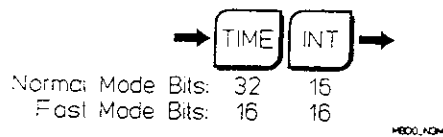
Figure 1A-B. Format 1A Binary Output
