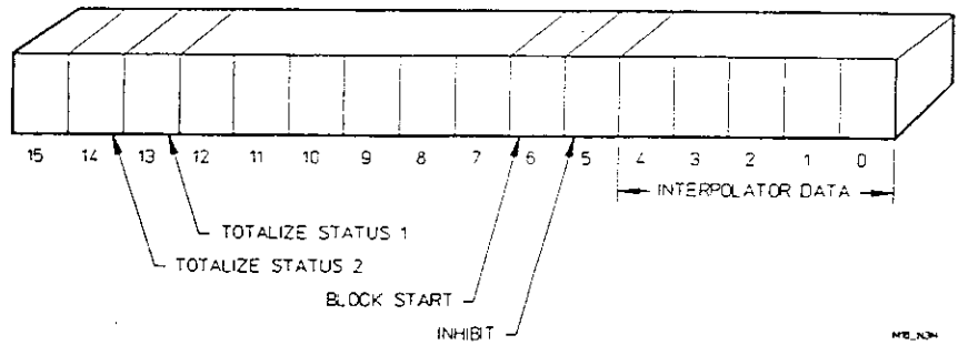
Figure 3-5. 16-bit Interpolator/Status Field
