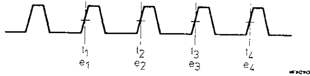
Figure 2A-D. Time Deviation and Phase Deviation Example Signal showing Time and Event Stamp Measurement Points.
