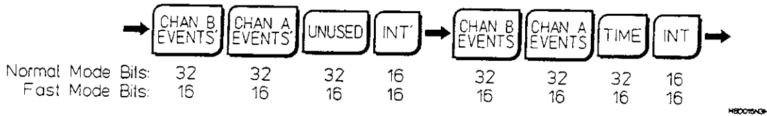
Figure 13-B. Format 13 Binary Output
