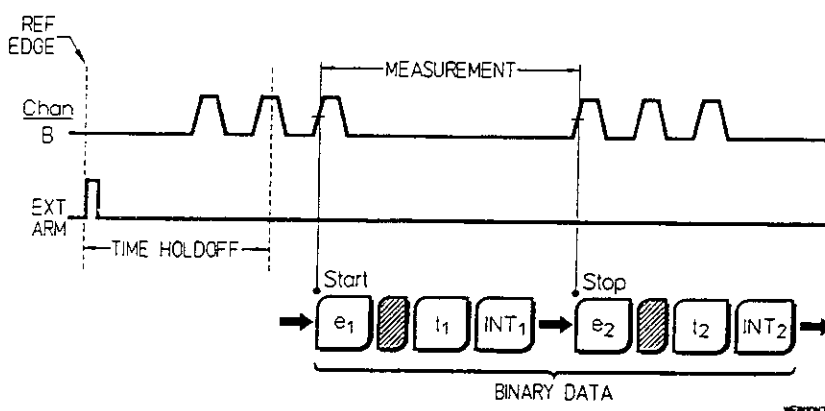
Figure 8-A. Time Interval Measurement on Channel B With Time Holdoff Arming Mode Showing Corresponding Binary Output.
