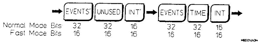
Figure 11-B. Format 11 Binary Output
